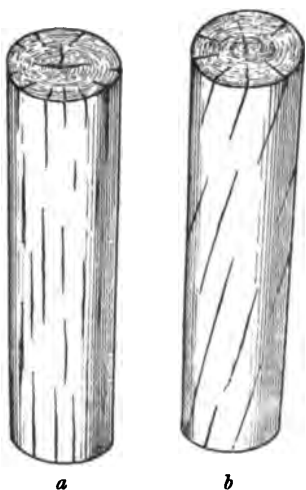
Fig. 57.—( a ) Straight-fibred stem with air-cracks on its surface and heart-shake on its transverse section. ( b ) Torse-fibred stem, ditto, also with wind-shake on its transverse section.
